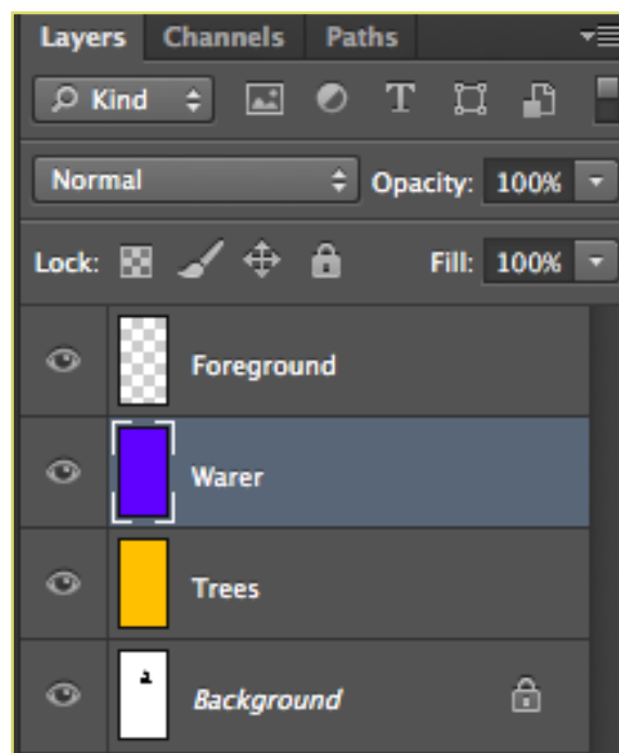
Figure 9. Layer palette
