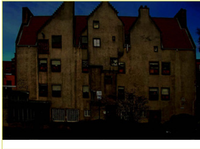
Figure 31. Underexposed photo
